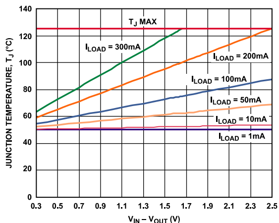
Figure 33. 500 mm² of PCB Copper, T_A = 50^\circ\text{C}
