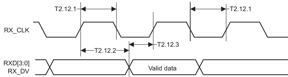
Figure 4-13. 10-Mbps MII Receive Timing
