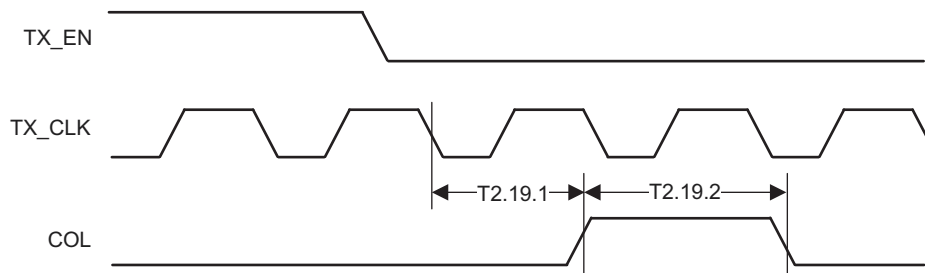
Figure 4-20. 10-Mbps Heartbeat Timing
