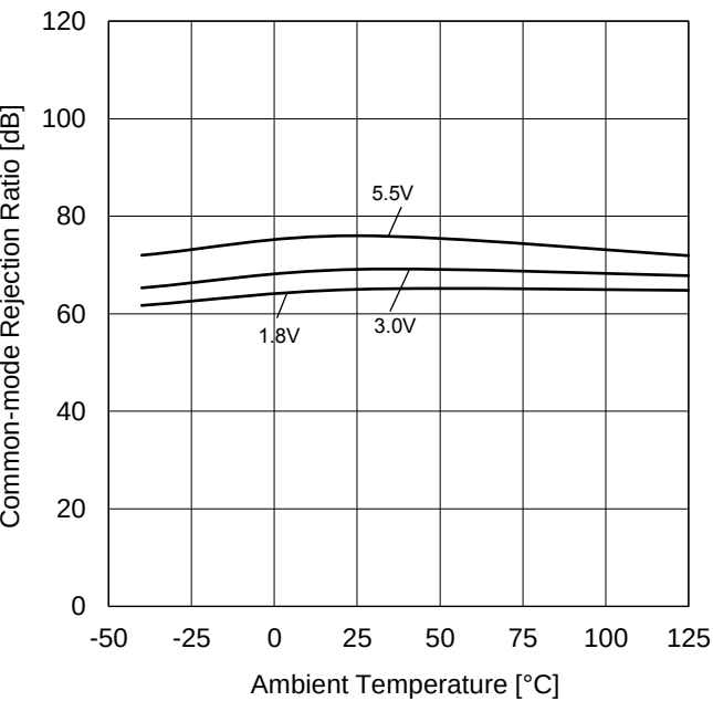
Figure 25. Common-mode Rejection Ratio vs Ambient Temperature
