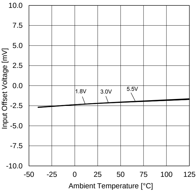
Figure 18. Input Offset Voltage vs Ambient Temperature ( V_{ICM}=V_{DD} , E_K=-V_{DD}/2 )
