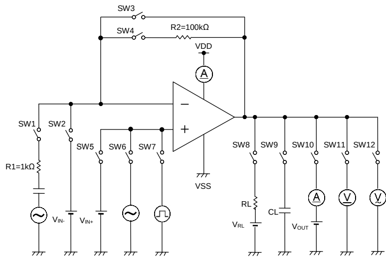
Figure 31. Test Circuit 2
