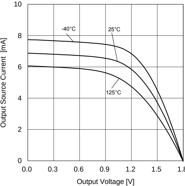
Figure 9. Output Source Current vs Output Voltage (V DD =1.8 V)
