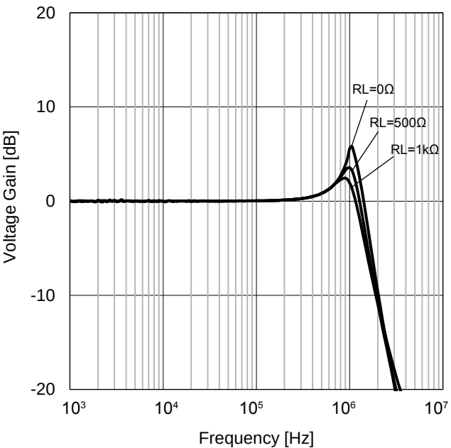
Figure 41. Voltage Gain vs Frequency (V DD =3.0 V, G V =0 dB, C L =100 pF, Circuit: Figure39)
