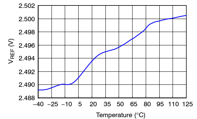
Figure 11. V_{REF} vs. Temperature
