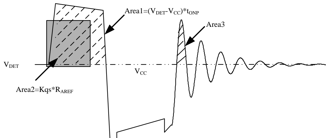
Figure 3. AREF Function
