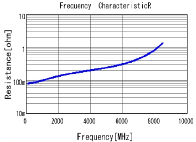
■ GCQ1555C1H7R0CB01 R DC0V, 25degC
