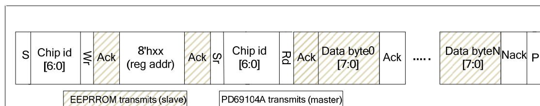
Figure 11: I2C EEPROM High Level Packet Structure.
