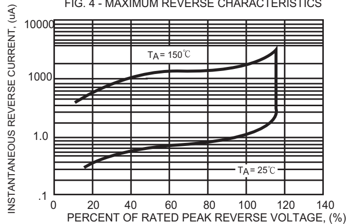
FIG. 4 - MAXIMUM REVERSE CHARACTERISTICS
