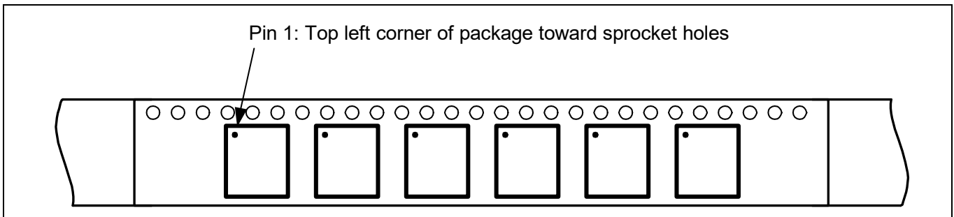
Figure 17 Pin 1 orientation
