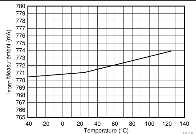
Figure 7-18. Port Current ADC Measurement (770mA) vs Temperature
