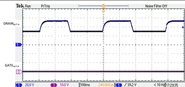
Figure 10-5. Open Circuit Detection Signature
