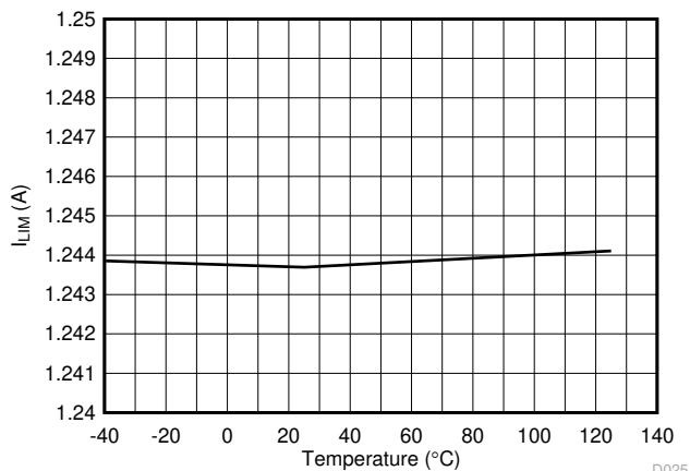
Figure 7-23. 2x Mode (2xFBn = 1) Current Limit vs Temperature
