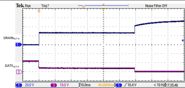
Figure 10-3. I_{LIM} Foldback and Turn-Off
