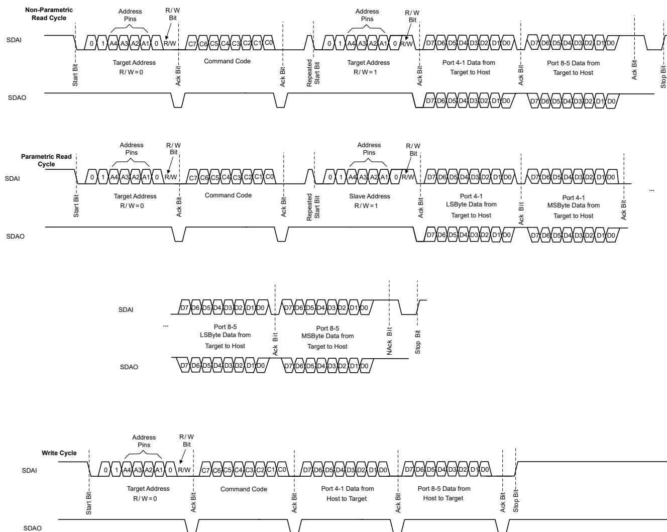
Figure 9-5. I²C interface Read and Write Protocol – Configuration B
