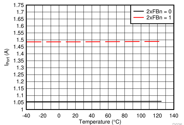
Figure 7-24. I_{\text{SHORT}} Threshold vs Temperature
