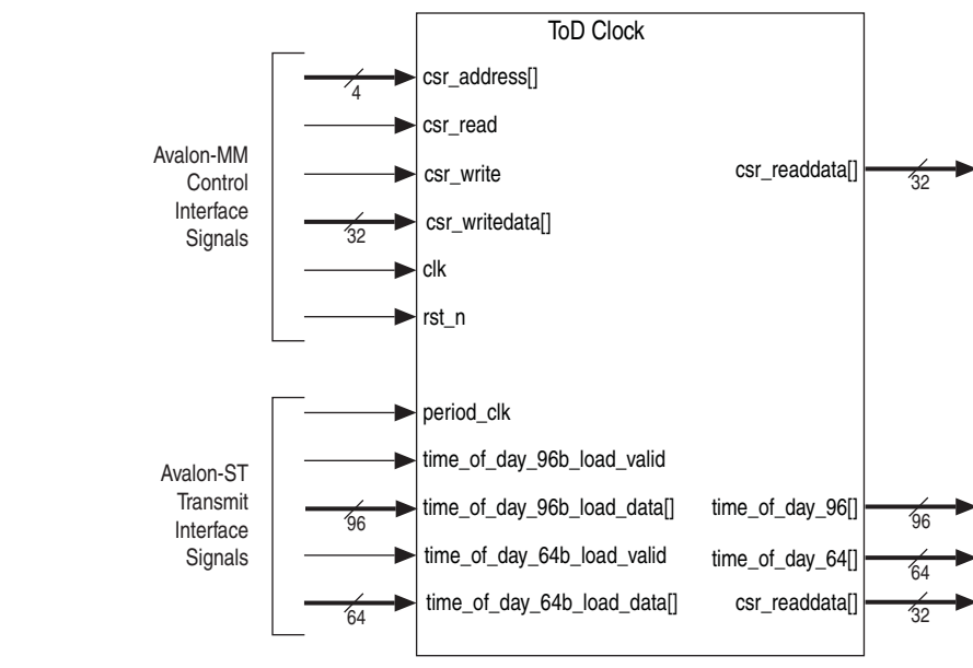
Figure B-1. ToD Clock Interface Signals
