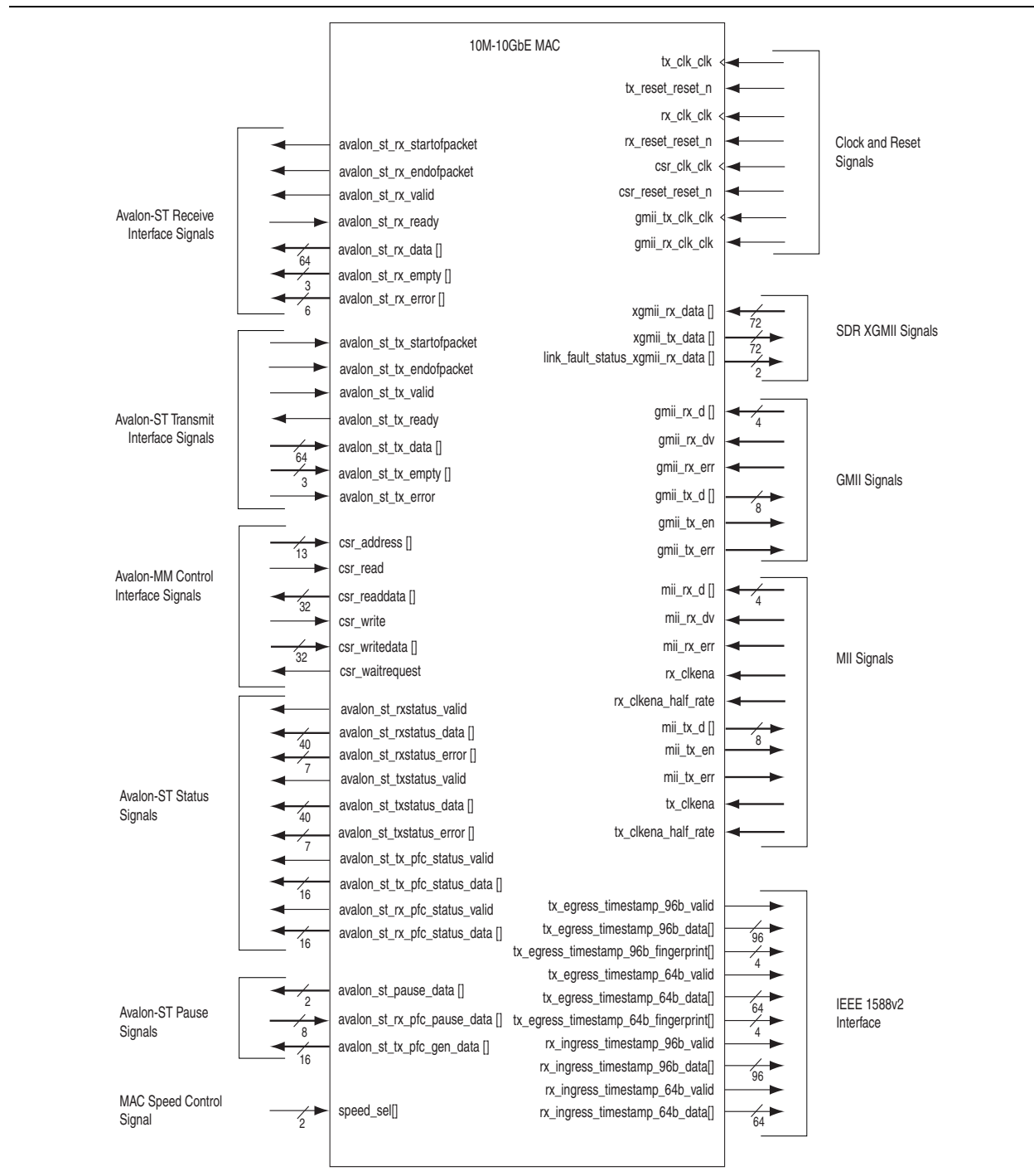
Figure 9–1. 10M-10GbE MAC
