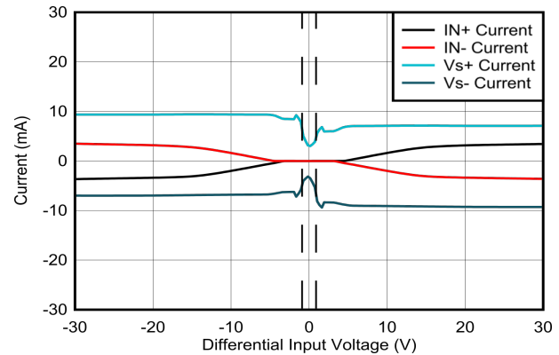
Figure 8-8. Current Consumption versus Differential Input Voltage
