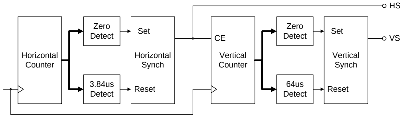
Figure 7. VGA display controller block diagram.
