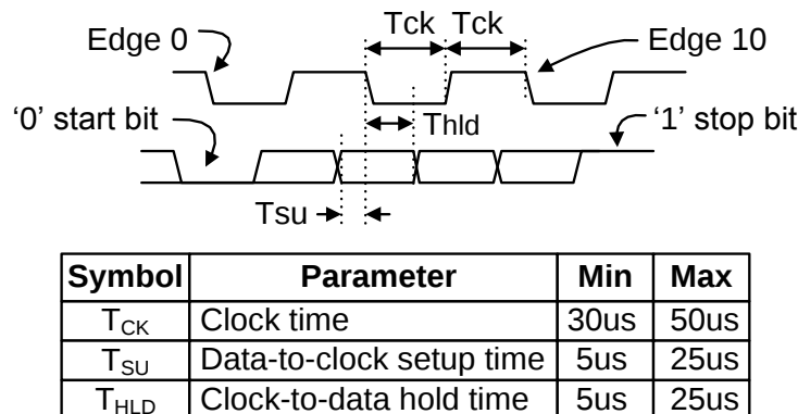
Figure 10. PS/2 Timing Diagram.
