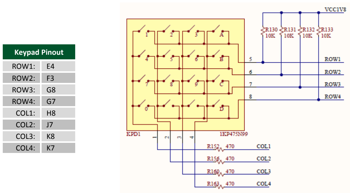
Figure 13. Keypad schematic
