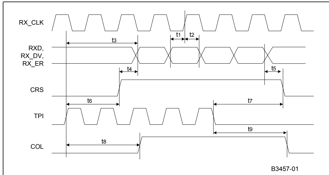
Figure 24 10BASE-T Receive Timing
