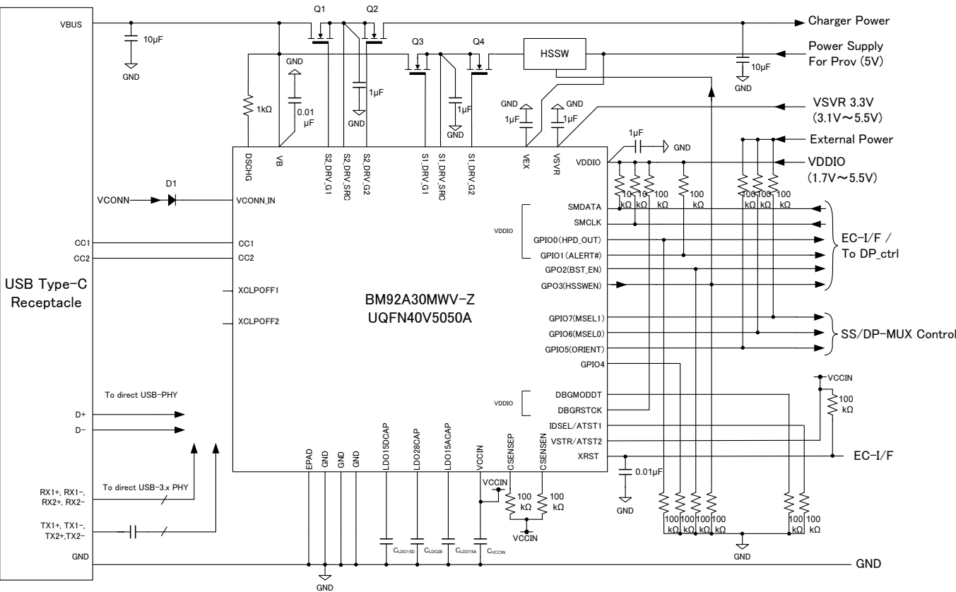
Figure 5-1 Application Example
