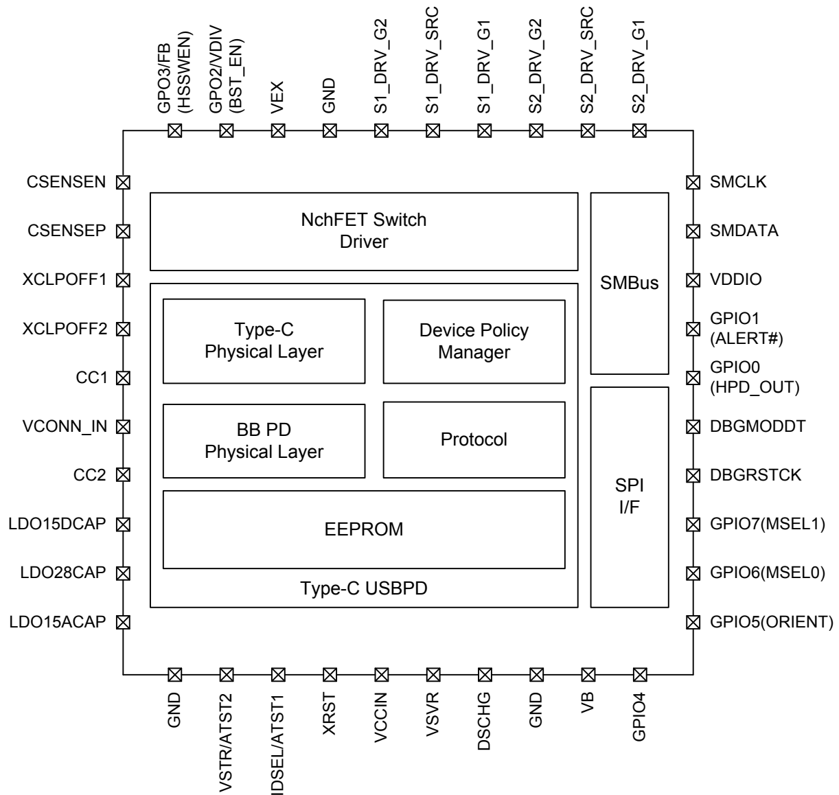
Figure 3-1 Block Diagram
