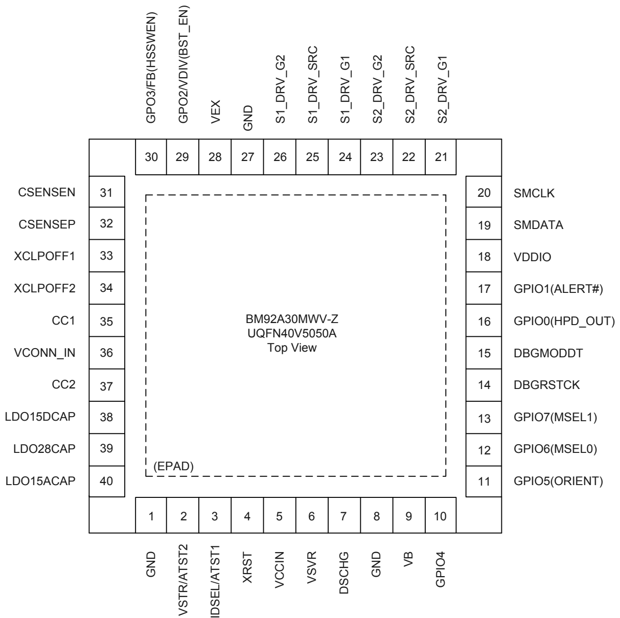
Figure 1-1 Pin configuration
