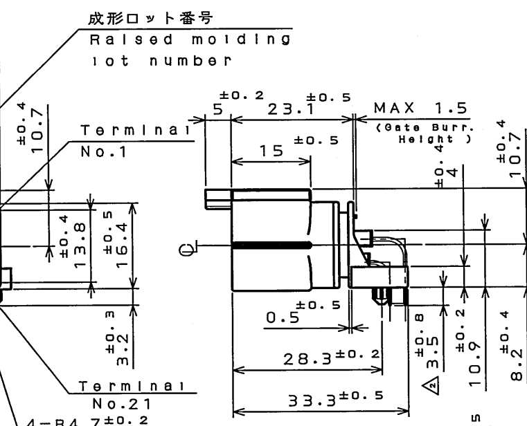
DETAIL C (SCALE 5:1)
