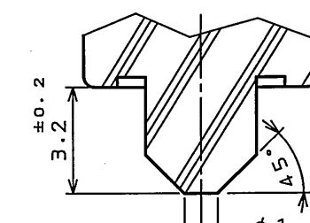
SECT. D-D (SCALE 5:1)
