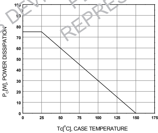
Figure 11. Power Derating
