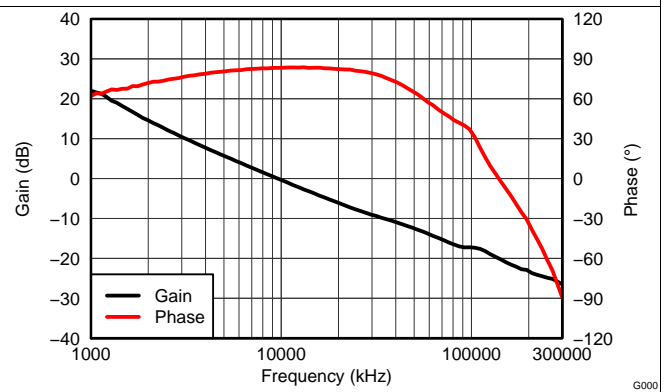
Figure 28. V_{IN} = 12\text{ V} , V_{OUT} = -12\text{ V} , I_{OUT} = 0.8\text{ A} , C_{OUT} = 4 \times 22\text{ }\mu\text{F} ceramic, f_{SW} = 800\text{ kHz}
