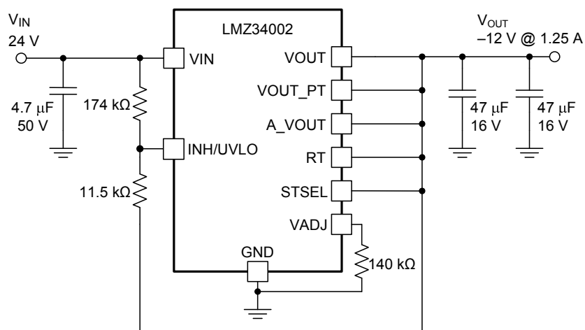
Figure 34. Typical Schematic V_{IN} = 24\text{ V} , V_{OUT} = -12\text{ V}
