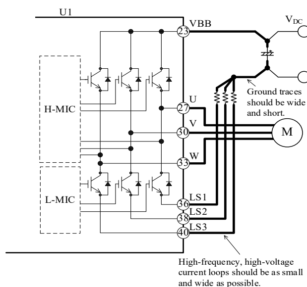
Figure 13-1. High-frequency, High-voltage Current Paths
