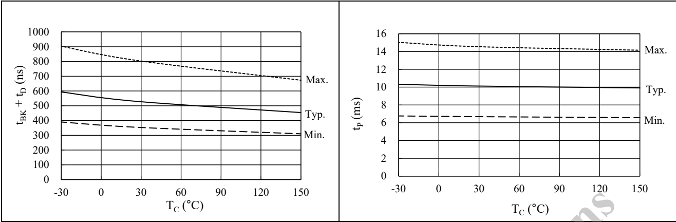
Figure 15-19. OCP Blanking Time, t_{BK(OC)} + t_{D(OC)} vs. T_C
