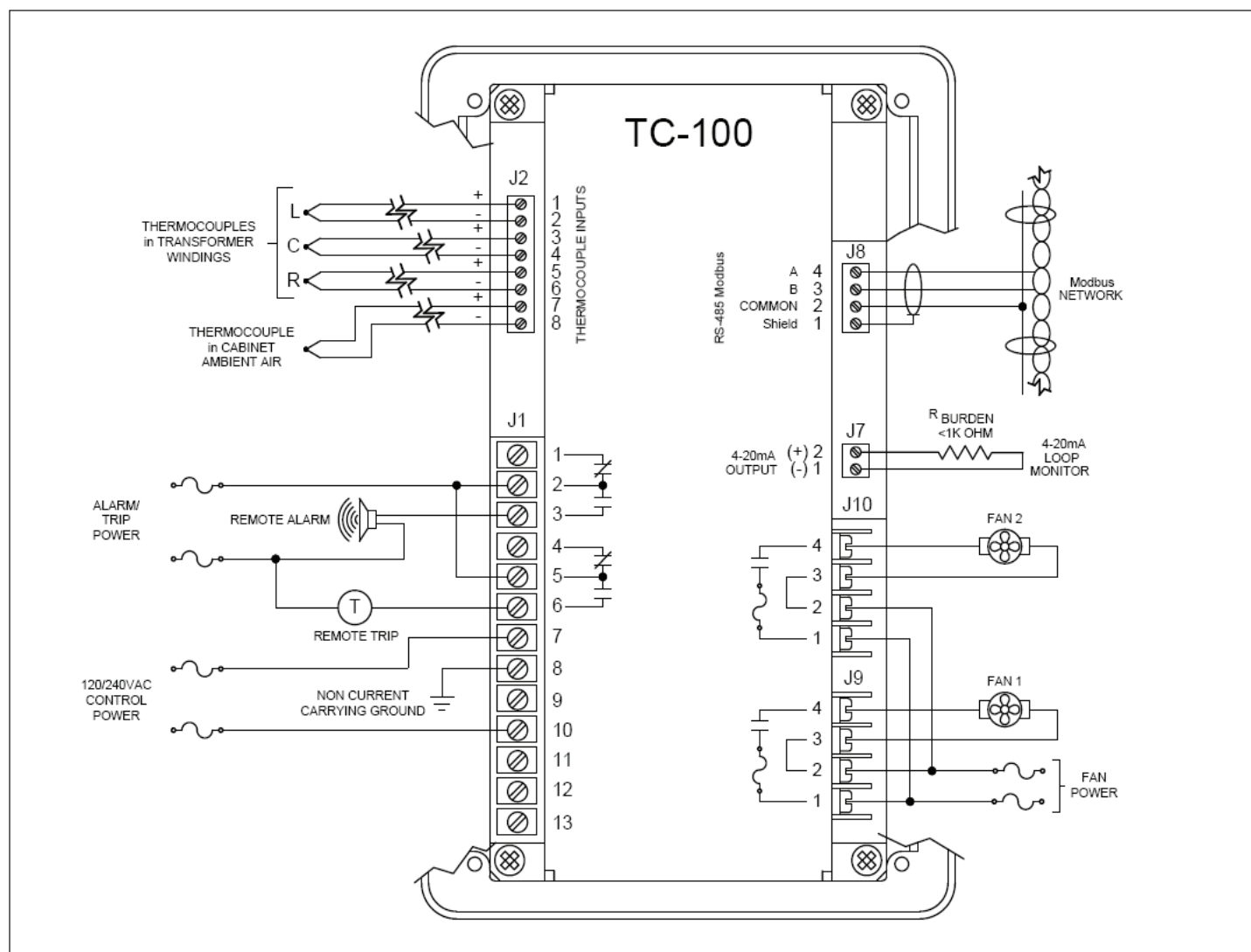
Figure 3. External Wiring
