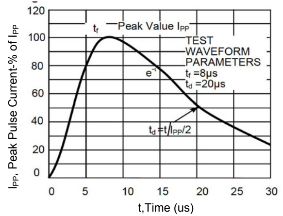
Figure 2. Pulse Waveform
