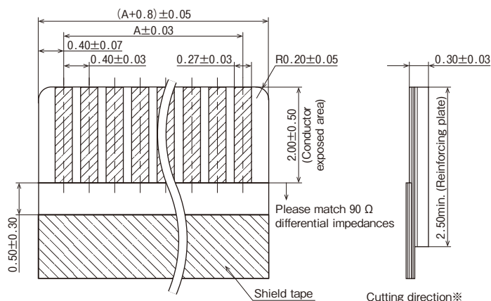
Applicable FFC dimensions (The conductive portions should be base by Ni plating and then Au plating.)
