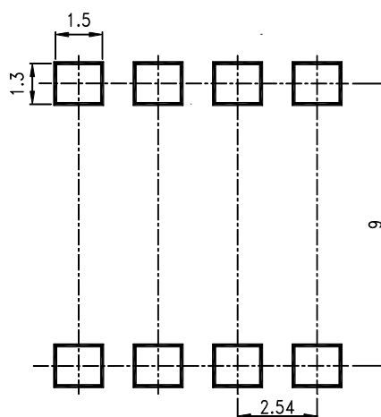
8 PIN
