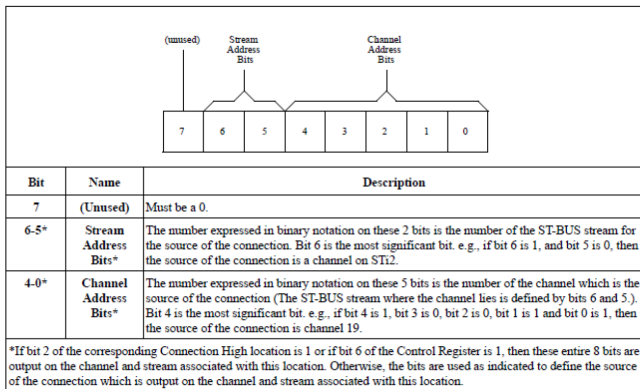
Figure 6 - Connection Memory Low Bits
