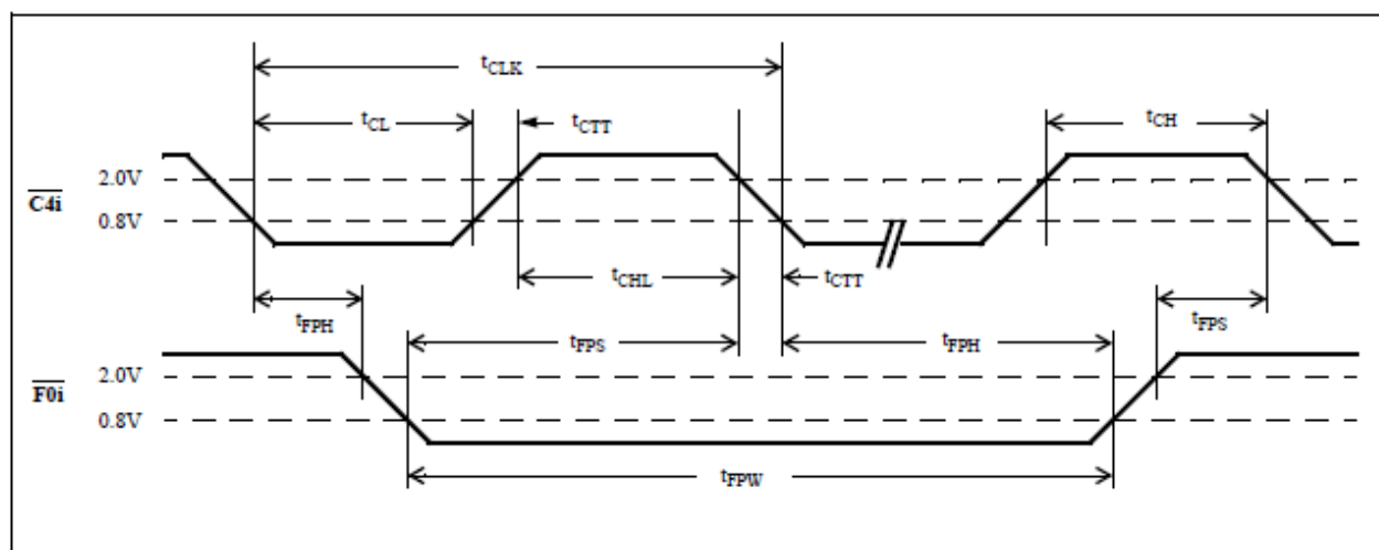
Figure 13 - Clock Timing
