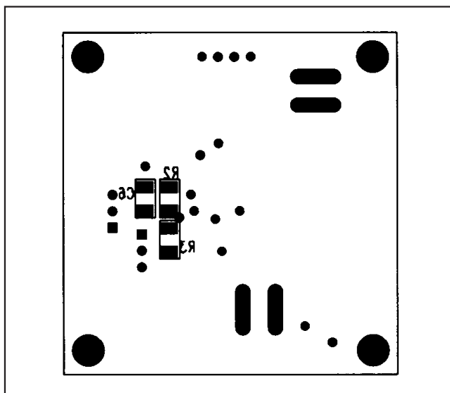
Figure 4. MAX1771 EV Kit PC Board Layout—Component Side
