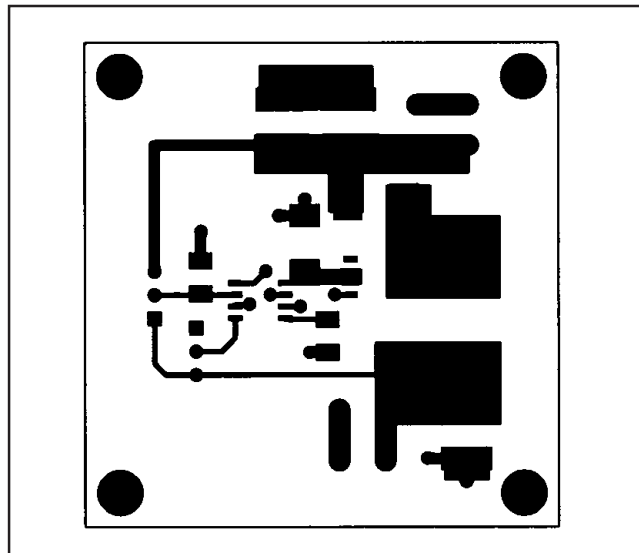
Figure 3. MAX1771 EV Kit Component Placement Guide—Solder Side
