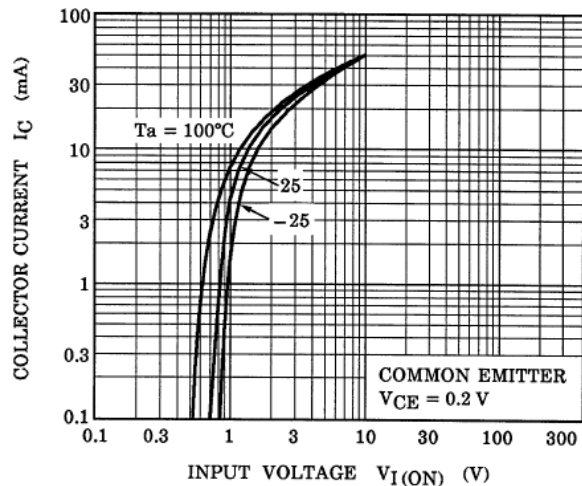
Fig. 10.1 RN1907 I_C - V_{I(ON)}
