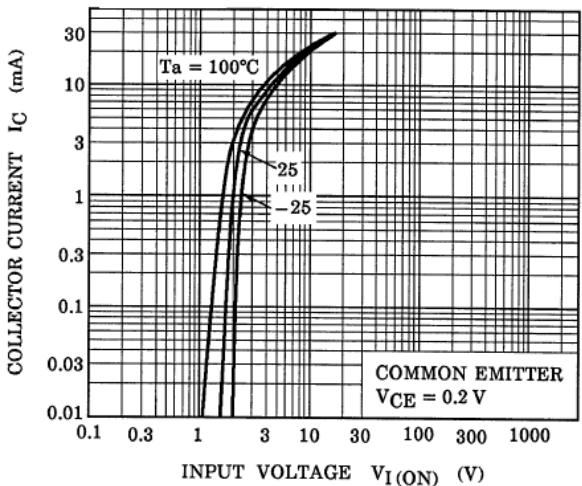
Fig. 10.3 RN1909 I_C - V_{I(ON)}
