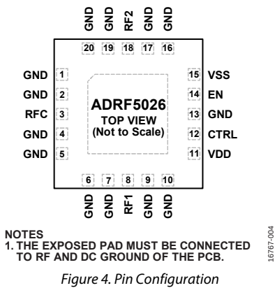
Figure 4. Pin Configuration
