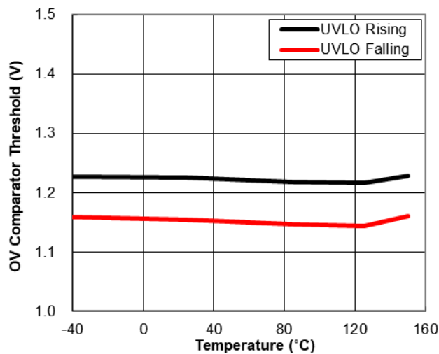
OVLO Comparator Threshold vs Temperature
