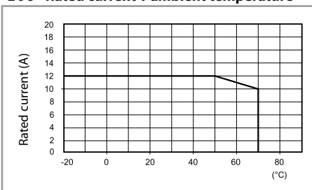
L 96 - Rated current v ambient temperature
