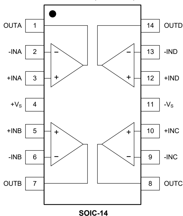
SGM8210-4 (TOP VIEW)
