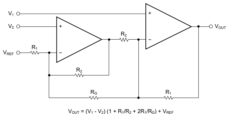
Figure 8. Low Power Instrumentation Amplifier Consisting of Two Operational Amplifiers
