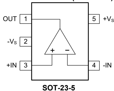
SGM8210-1AXN5G (TOP VIEW)
