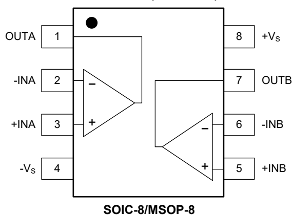
SGM8210-2 (TOP VIEW)
