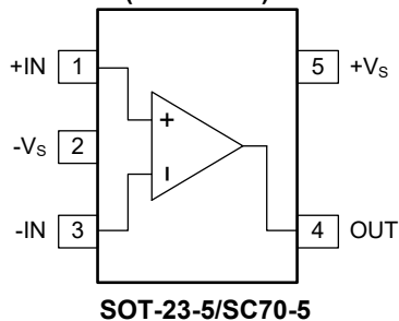
SGM8210-1BXN5G/SGM8210-1XC5G (TOP VIEW)
