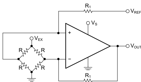
Figure 5. Bridge Amplifier Using a Single Operational Amplifier
