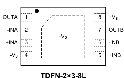
SGM8210-2 (TOP VIEW)
