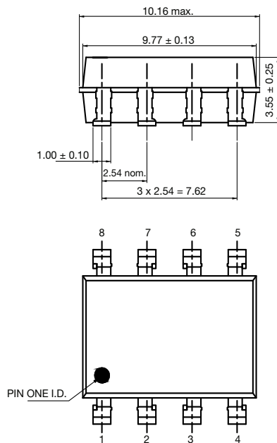
DIP-8 (option 9)
