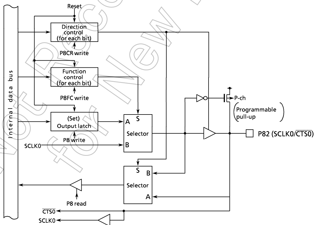
Figure 3.5 (27) Port 8 (P82)
