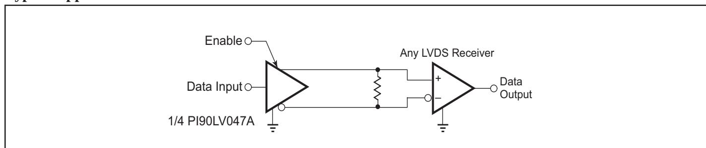
Figure 6. Point-to-Point Application
