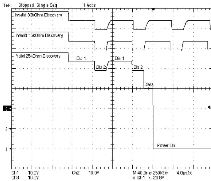
Figure 8. Invalid (33 k \Omega and 15 k \Omega ) and Valid Discovery (25 k \Omega )
