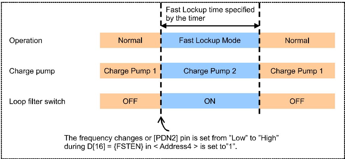
Fig. 6 Timing Chart for Fast Lockup Mode
