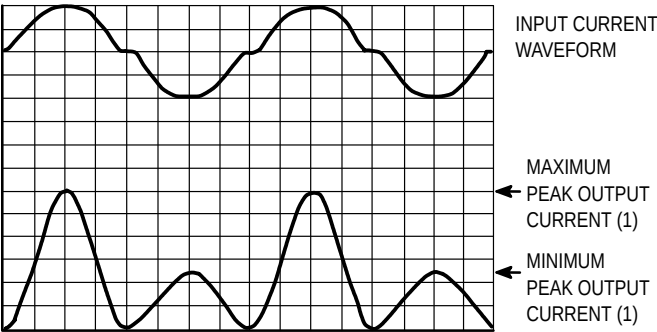
Figure 2. Output Characteristics
