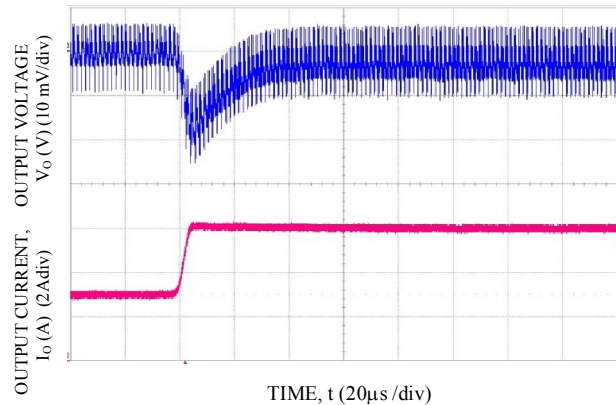
Transient Response to Dynamic Load Change from 50% to 100% at 12Vin, Cout-1x47 \mu F+3x330 \mu F, CTune-12nF & RTune-178. V_o =1.2V
