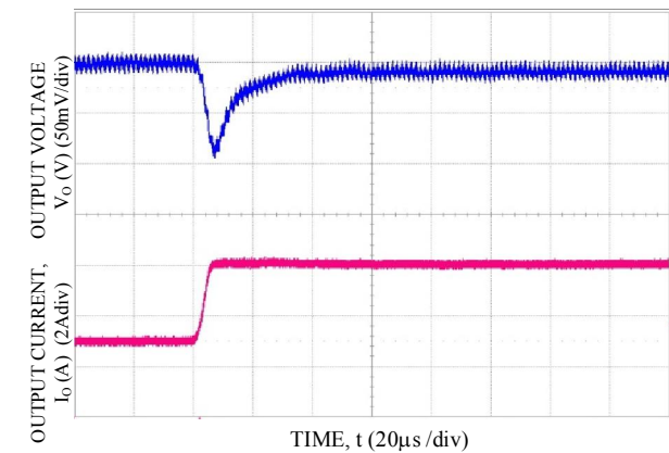
Transient Response to Dynamic Load Change from 50% to 100% at 12Vin, Cout-2x47 \mu F, CTune-2200pF & RTune-261. V_o =5V
