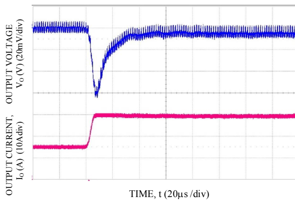
Transient Response to Dynamic Load Change from 50% to 100% at 12Vin, Cout-3x47 \mu F, CTune-3900pF & RTune-178. V_o =3.3V
