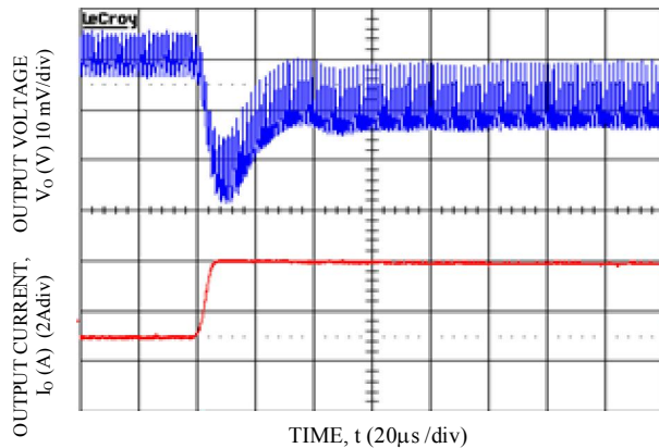
Transient Response to Dynamic Load Change from 50% to 100% at 8Vin, Cout-1x47 \mu F+4x330 \mu F, CTune-33nF, RTune-178. V_o =0.6V
