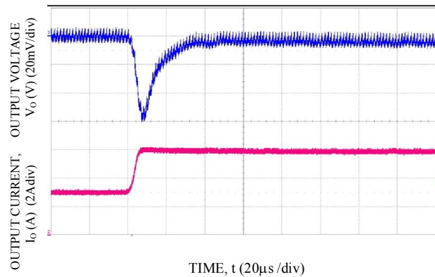
Transient Response to Dynamic Load Change from 50% to 100% at 12Vin, Cout-3x47 \mu F, CTune-3300pF & RTune-178. V_o =2.5V
