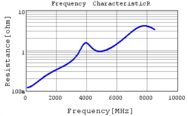
GRM1555C2A220JA01 R DCOV, 25degC
