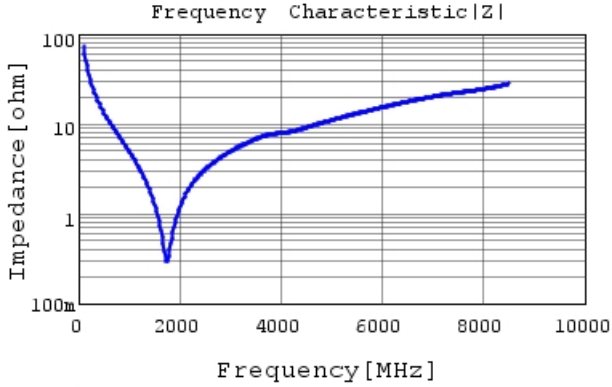
GRM1555C2A220JA01 |Z| DCOV, 25degC
