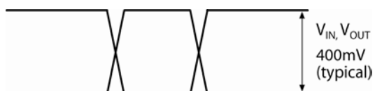
Figure 3a. Single-Ended Swing
