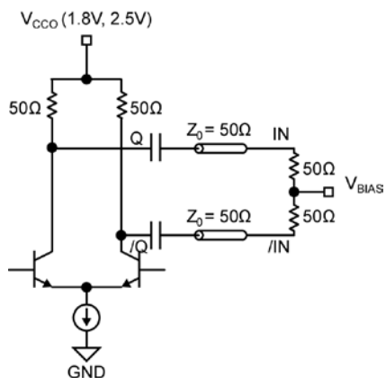
Figure 5c. CML AC-Coupled Termination. VCCO 1.8V, 2.5V only.
