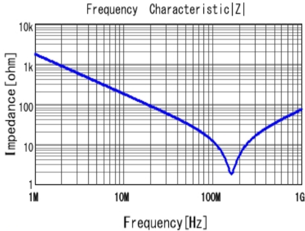
■ DE1B3RB101KN4AR01F |Z| DC0V, 20degC
