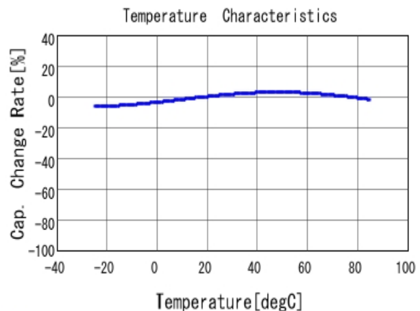
■ DE1B3RB101KN4AR01F C-Temp. capchange, DC0V, AC1Vrms
