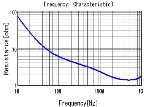
■ DE1B3RB101KN4AR01F R DC0V, 20degC
