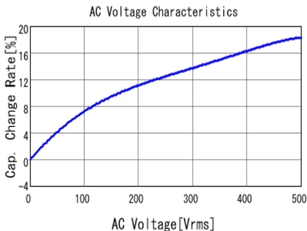
■ DE1B3RB101KN4AR01F C-AC Voltage capchange, DC0V, 20.0
