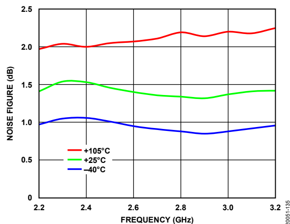
Figure 37. Noise Figure vs. Frequency at Various Temperatures
