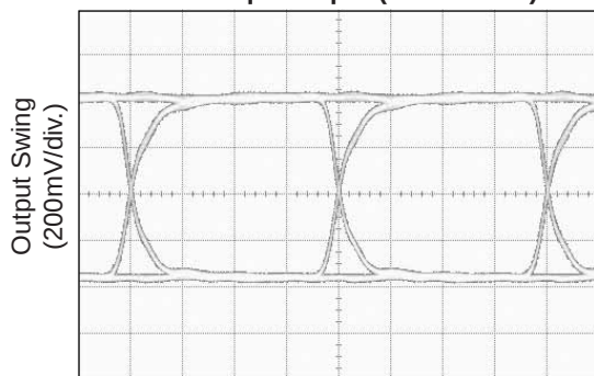
1.25Gbps Output ( 2^{23}-1 PRBS)
