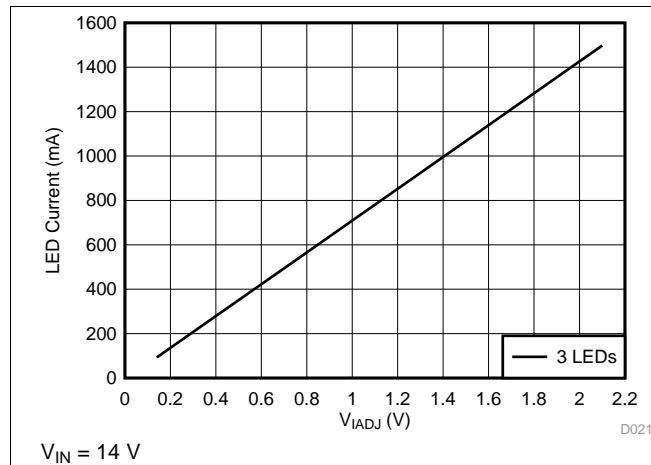
Figure 55. LED Current vs IADJ Voltage
