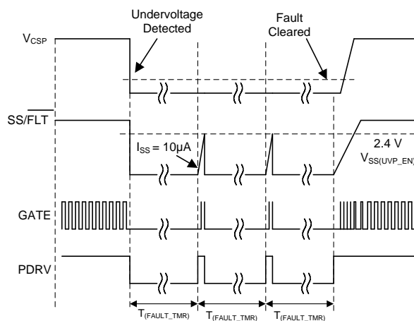
Figure 33. Output Undervoltage Fault Protection
