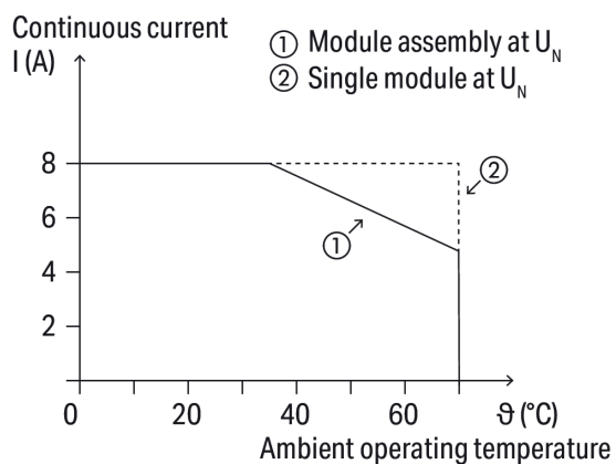
Current-carrying capacity curve
