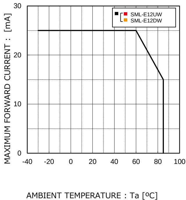
Fig.4 Derating
