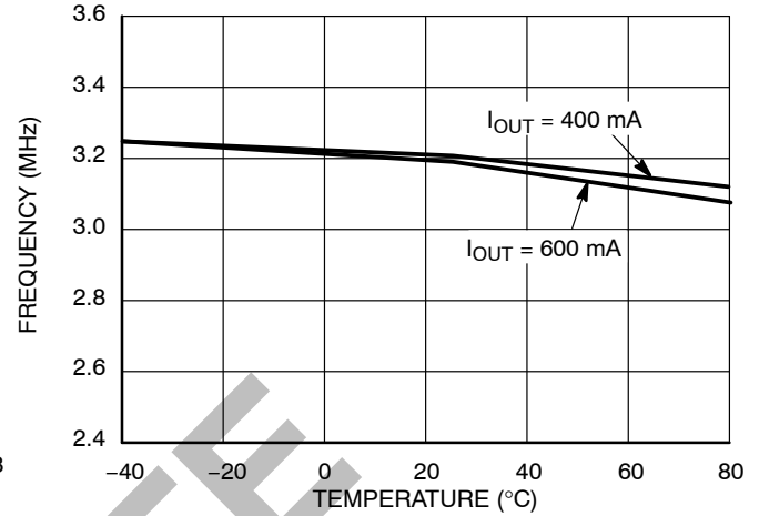
Figure 10. Frequency vs. Temperature
