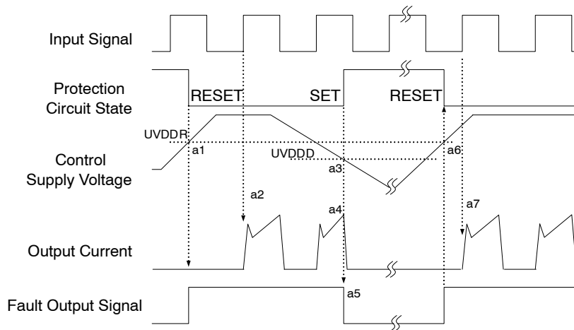
Figure 6. Under-Voltage Protection
