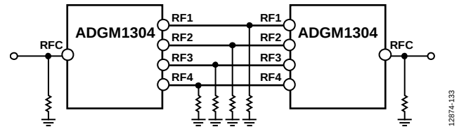
Figure 67. Two ADGM1304 Devices Connected in Path Selection Configuration with 10 M \Omega Shunt Resistors to Mitigate Floating Nodes
