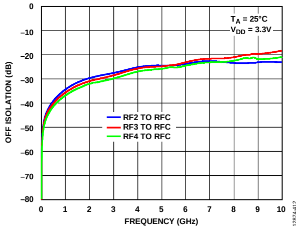
Figure 18. Off Isolation vs. Frequency, RF1 to RFC On ( V_{DD} = 3.3\text{ V} )
