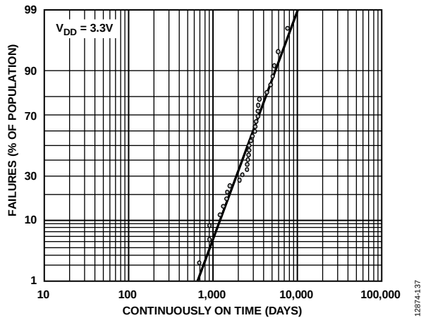
Figure 69. Cumulative On Switch Lifetime at 50°C, V_{DD} = 3.3V , Sample Size = 31 Devices
