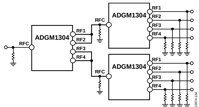
Figure 68. Three ADGM1304 Devices Connected in Fanout Configuration with 10 M \Omega Shunt Resistors to Mitigate Floating Nodes
