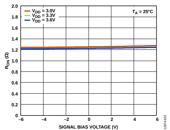
Figure 11. R_{ON} vs. Signal Bias Voltage over Supply Voltages (Measured 5 sec Post Switch Turn On Time, RF1 to RFC On)
