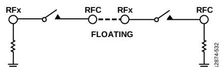
Figure 65. RFC Connected to RFx
