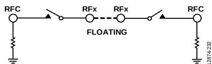
Figure 64. RFx Pins of Two MEMS Switches Directly Connected
