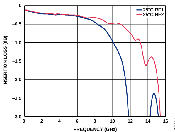
Figure 14. Insertion Loss vs. Frequency on Linear Scale ( V_{DD} = 3.3 V)
