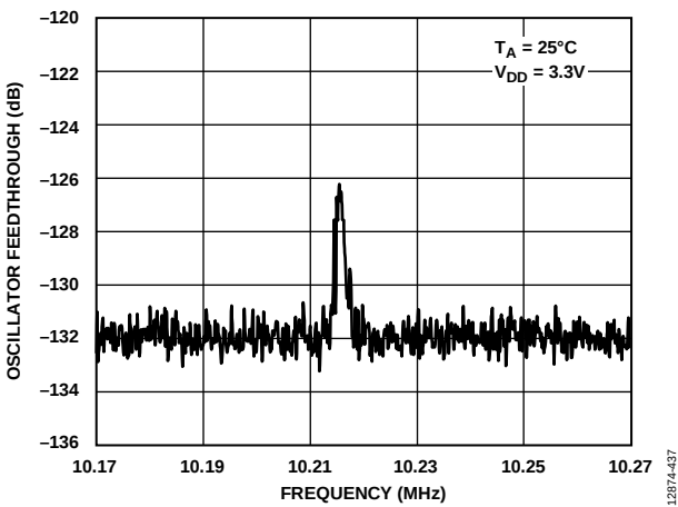
Figure 30. Oscillator Feedthrough, Zoomed In at 10.2 MHz
