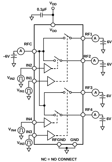
Figure 46. Off Leakage
