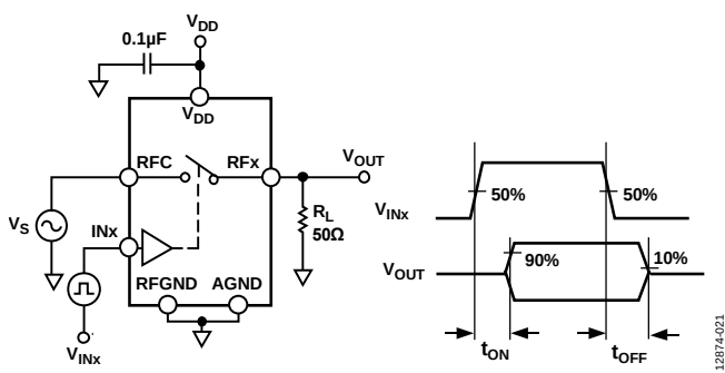
Figure 41. Switch Timings, t_{ON} and t_{OFF}
