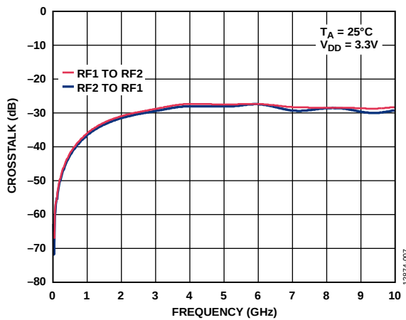
Figure 19. Crosstalk vs. Frequency ( V_{DD} = 3.3\text{ V} )
