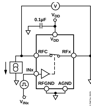
Figure 43. On Resistance
