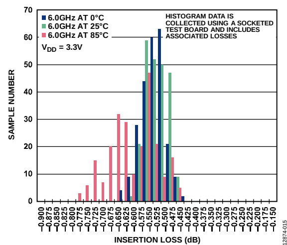
Figure 23. 6.0 GHz Insertion Loss Histogram at Various Temperatures, V_{DD} = 3.3\text{ V}
