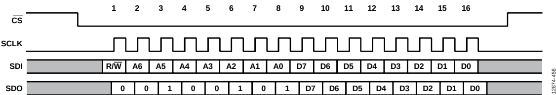
Figure 49. Addressable Mode Timing Diagram (Mode 0)
