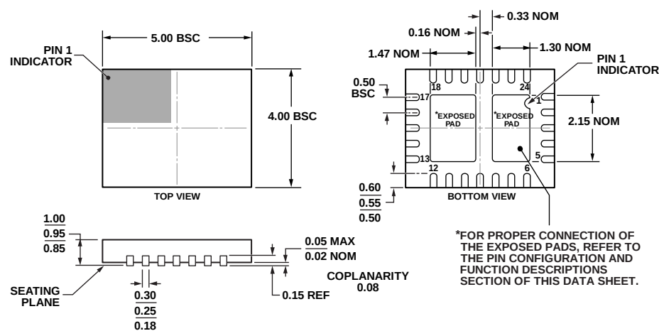
Figure 72. 24-Lead Lead Frame Chip Scale Package [LFCSP_VQ] 5 mm x 4 mm Body, Very Thin Quad (CP-24-9) Dimensions shown in millimeters
