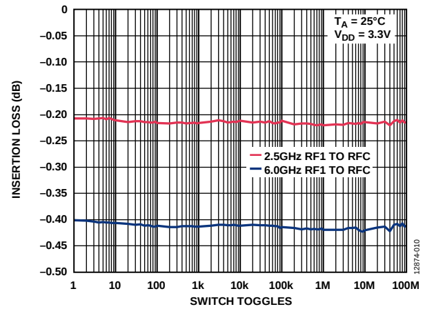
Figure 21. Insertion Loss vs. Switch Toggles ( V_{DD} = 3.3\text{ V} )
