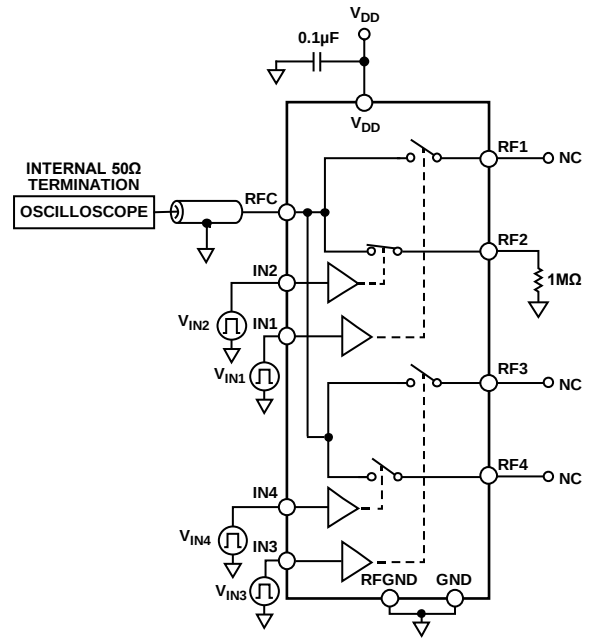
Figure 39. Video Feedthrough
