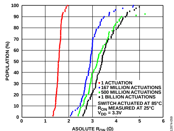
Figure 59. Population vs. Absolute R_{ON} Switch Actuated at 85^\circ\text{C} and R_{ON} Measured at 25^\circ\text{C}
