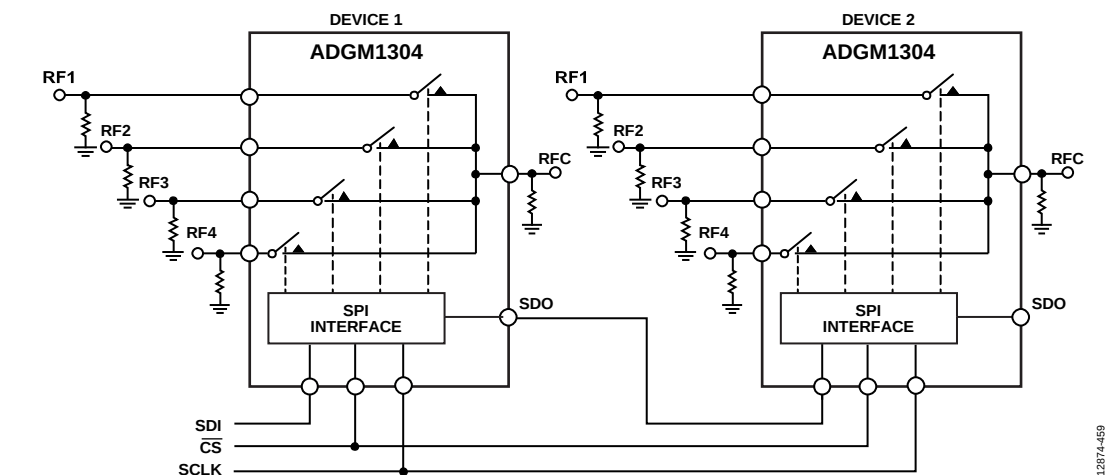
Figure 51. Two SPI-Controlled ADGM1304 Switches Connected in a Daisy-Chain Configuration
