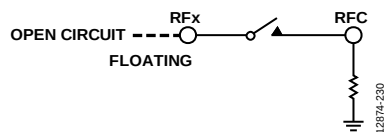
Figure 62. RFx Pins Left Open Circuit
