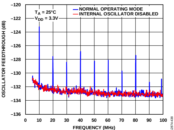
Figure 31. Oscillator Feedthrough Wide Bandwidth
