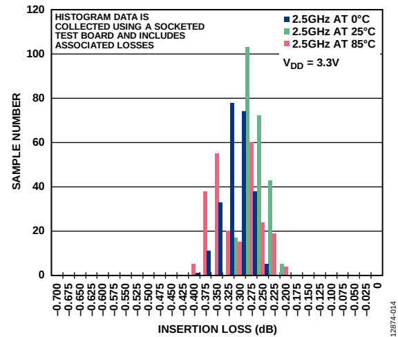
Figure 22. 2.5 GHz Insertion Loss Histogram at Various Temperatures, V_{DD} = 3.3\text{ V}
