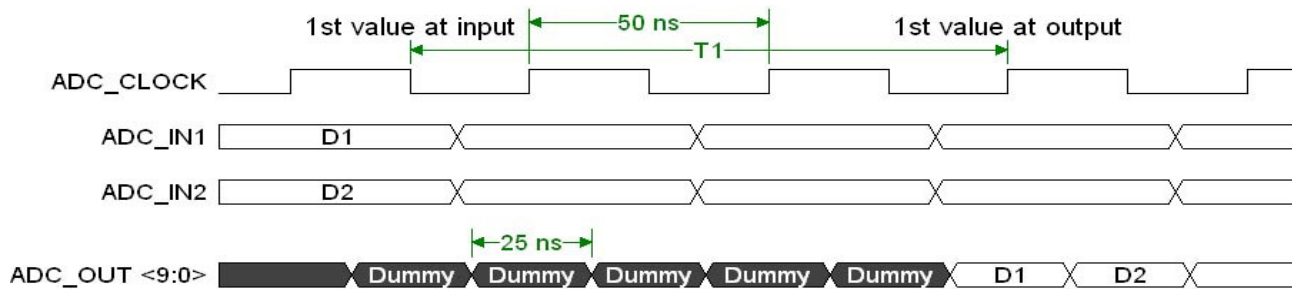
Figure 21. ADC Timing using Two Analog Outputs
