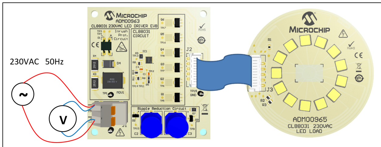
FIGURE 2-1: Connection Diagram.
